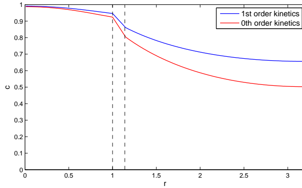
Figure 7: Comparison of solutions at z = 1 for first order kinetics (reaction rate linear in concentration) and zeroth-order kinetics (reaction rate constant). As in Figure 6, with the Péclet number Pe = 10 and the Damköhler number 0.1 in each case ( Da = 0.1 or Da_0 = 0.1 ).
